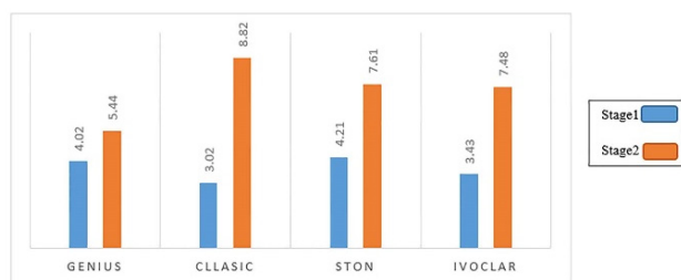
Figure 4. Mean Wear Rate of Specimens After First and Second Stages*
