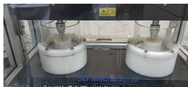
Figure 3. Chewing Simulator Machine.
