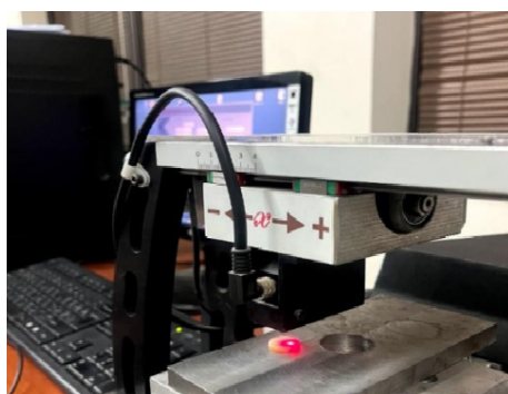
Figure 2. Surface Roughness Laser Check
